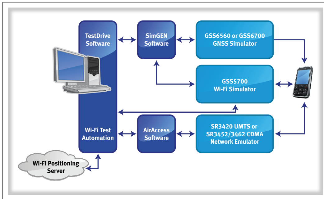
Spirent's Location Technology Solution with Integrated Wi-Fi Positioning.
