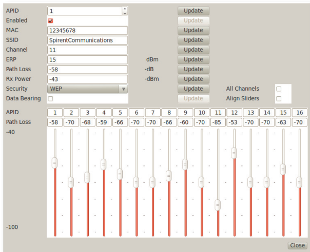
The GSS5700’s user interface allows full interactive control. (Typical remote user interface, subject to change).
